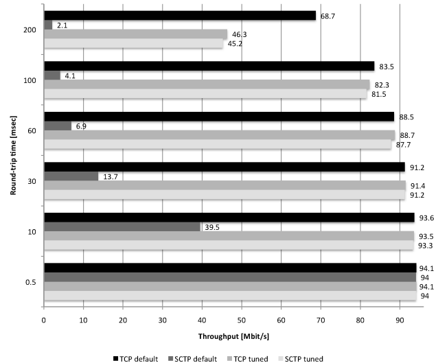
Fig. 4. Iperf measurements with default and tuned parameters
