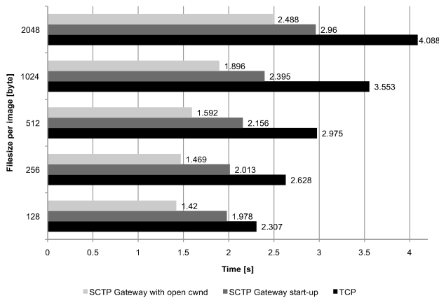
Fig. 5. Time required for a serial download of an HTML page with five images of the same size
