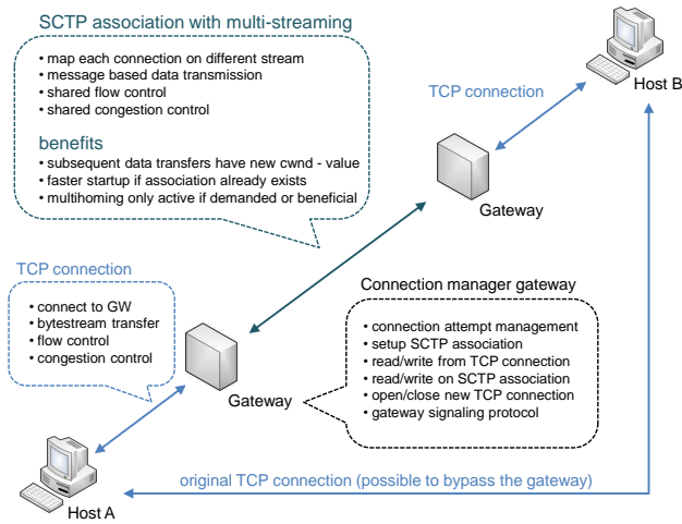
Fig. 2. The Connection Manager Gateway (CMG)
