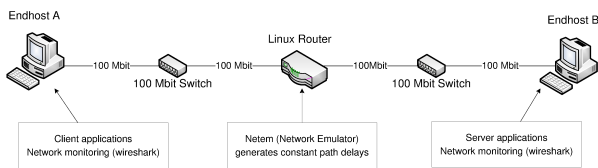
Fig. 3. Network testbed used for the practical measurements
