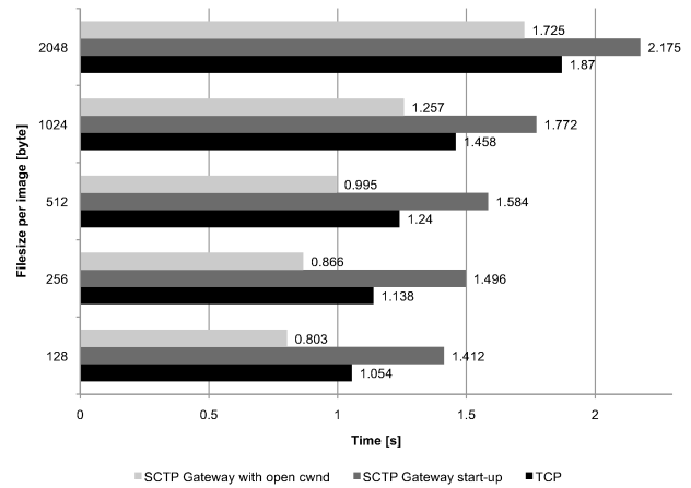
Fig. 6. Time required for a serial download of an HTML page with five images of the same size using persistent connections
