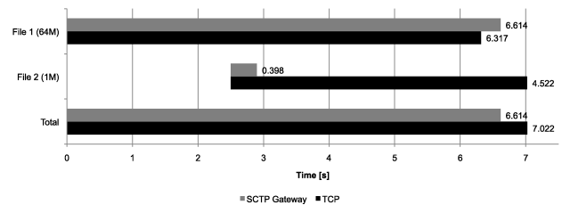
Fig. 7. Timeline of transferring two files when the longer transfer (file 1) is joined by a shorter one (file 2) after 2.5 seconds
