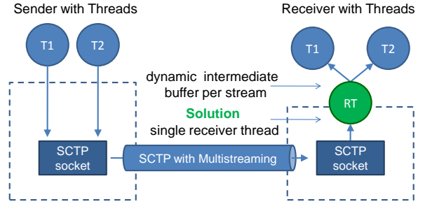
Fig. 1. Parallel transmissions with SCTP’s multi-streaming
