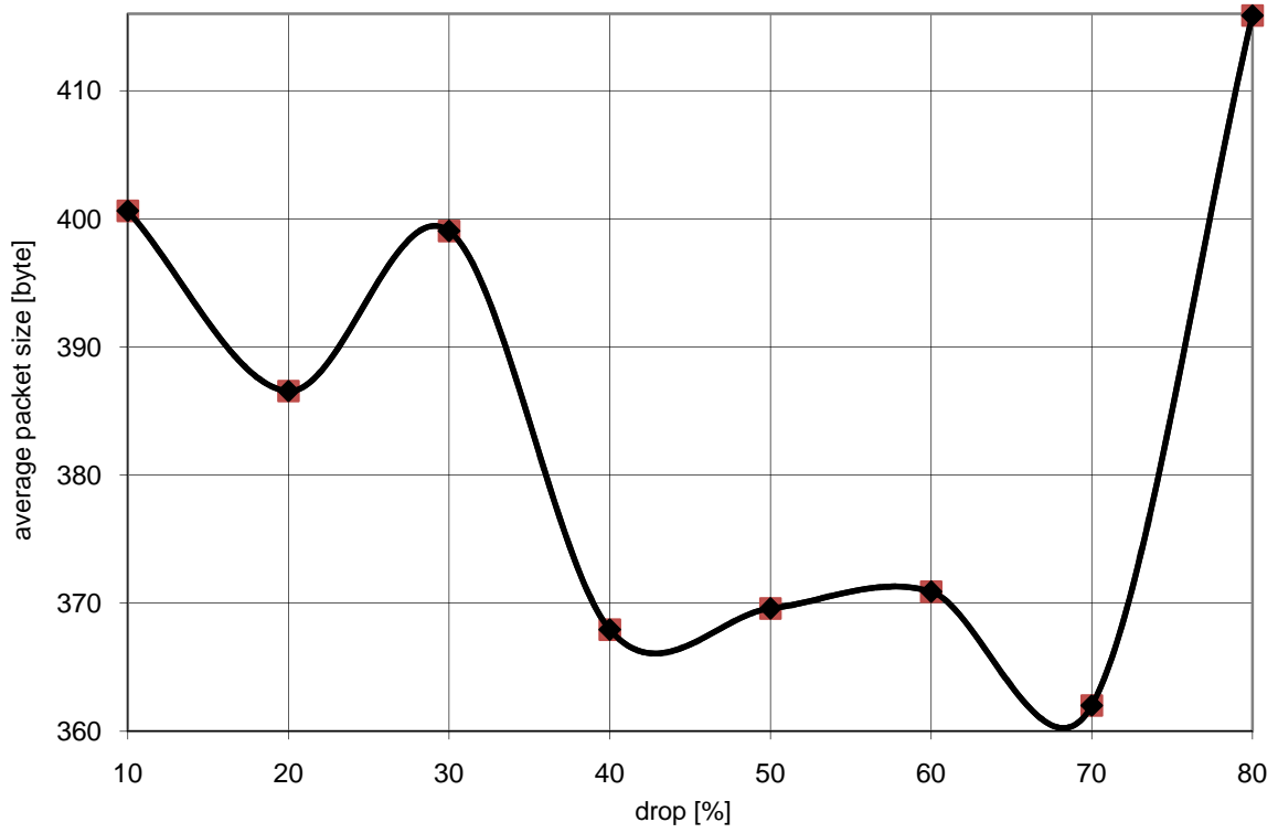
Diagramm b2_drop1: Battlefield 2 drop 1
