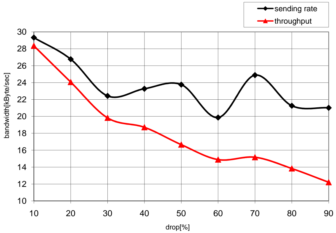
Diagramm a_drop3: Anno1701 drop 3
