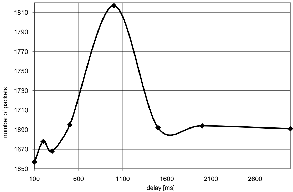
Diagramm q4_delay2: Quake 4 delay 2
