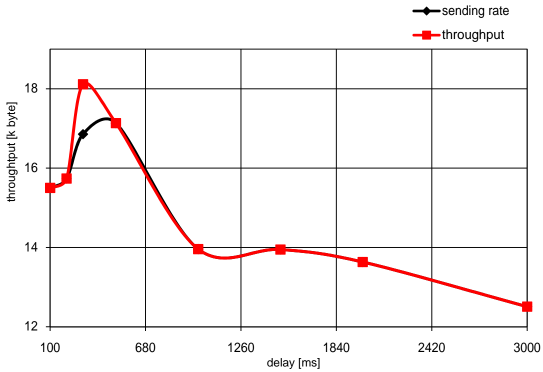
Diagramm aoe_delay3: Age of Empires delay 3
