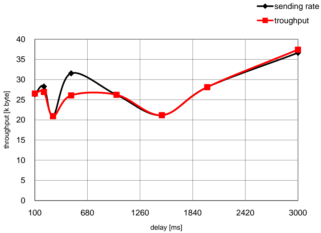
Diagramm a_delay3: Anno1701 delay 3
