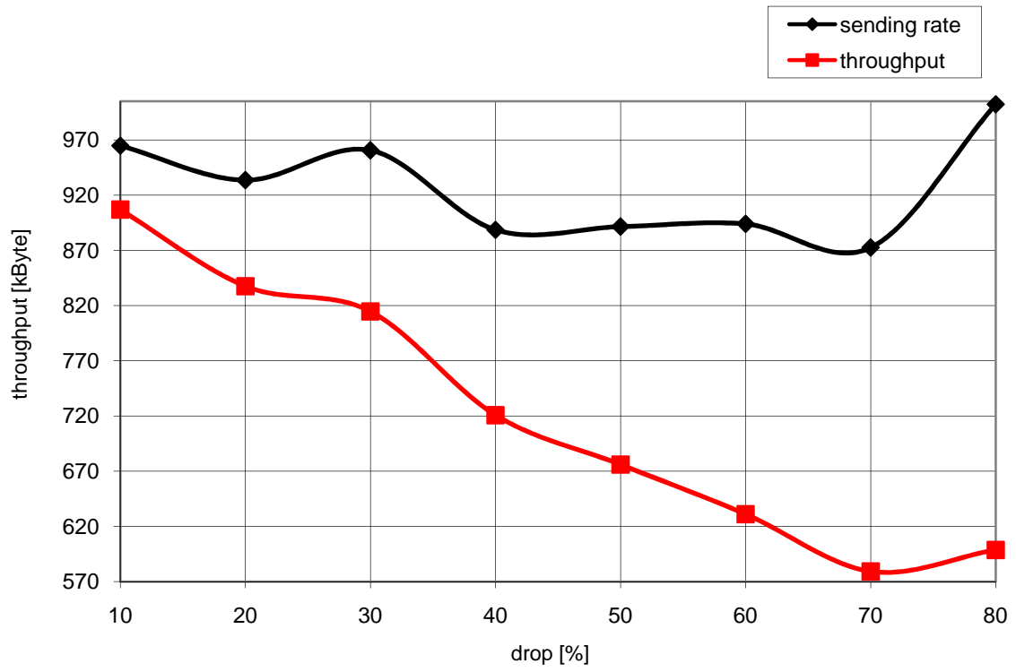
Diagramm b2_drop3: Battlefield 2 drop 3
