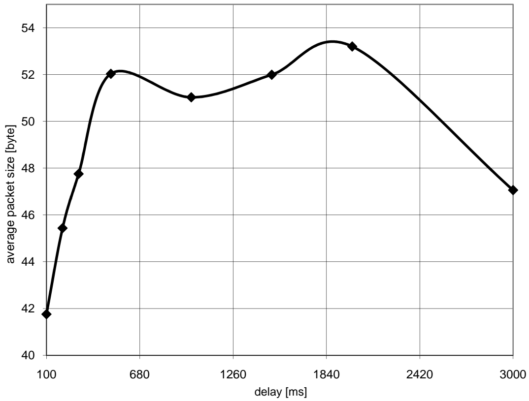
Diagramm dow_delay1: Dawn of War delay 1
