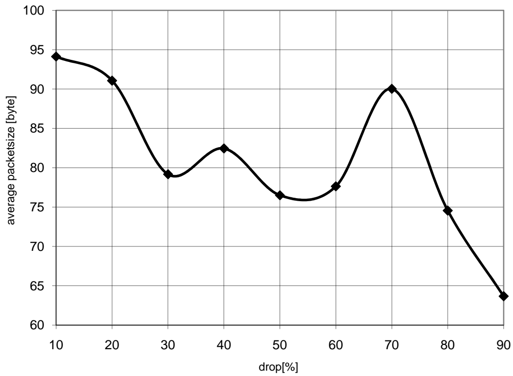
Diagramm a_drop1: Anno1701 drop 1
