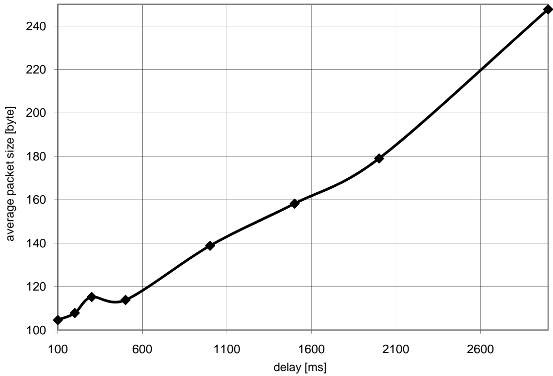
Diagramm q4_delay1: Quake 4 delay 1
