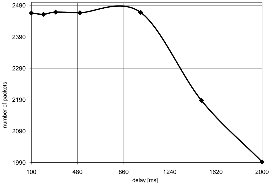
Diagramm b2_delay2: Battlefield 2 delay 2
