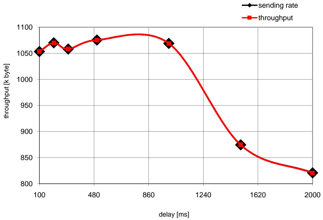
Diagramm b2_delay3: Battlefield 2 delay 3
