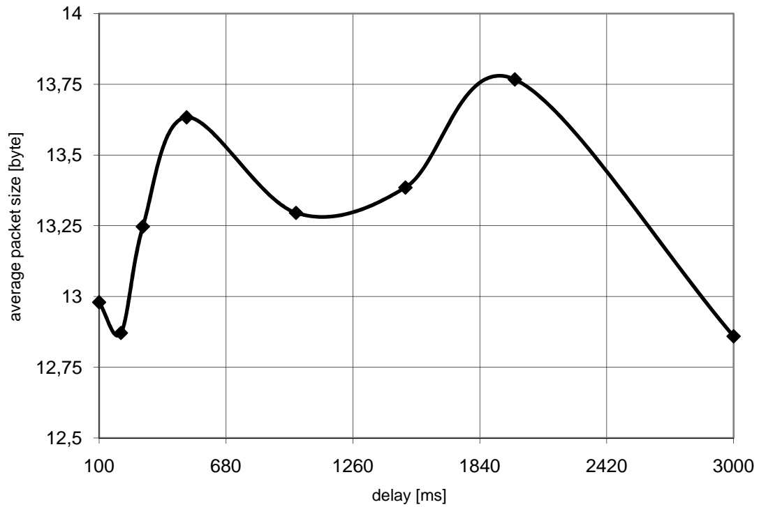
Diagramm aoe_delay1: Age of Empires delay 1
