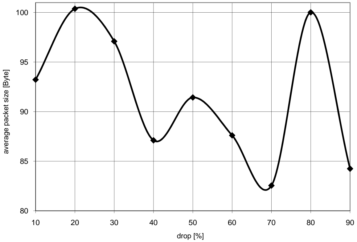
Diagramm q4_drop1: Quake 4 drop 1
