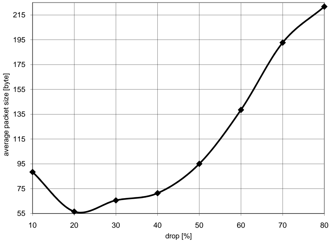
Diagramm fifa_drop1: Fifa 2007 drop 1
