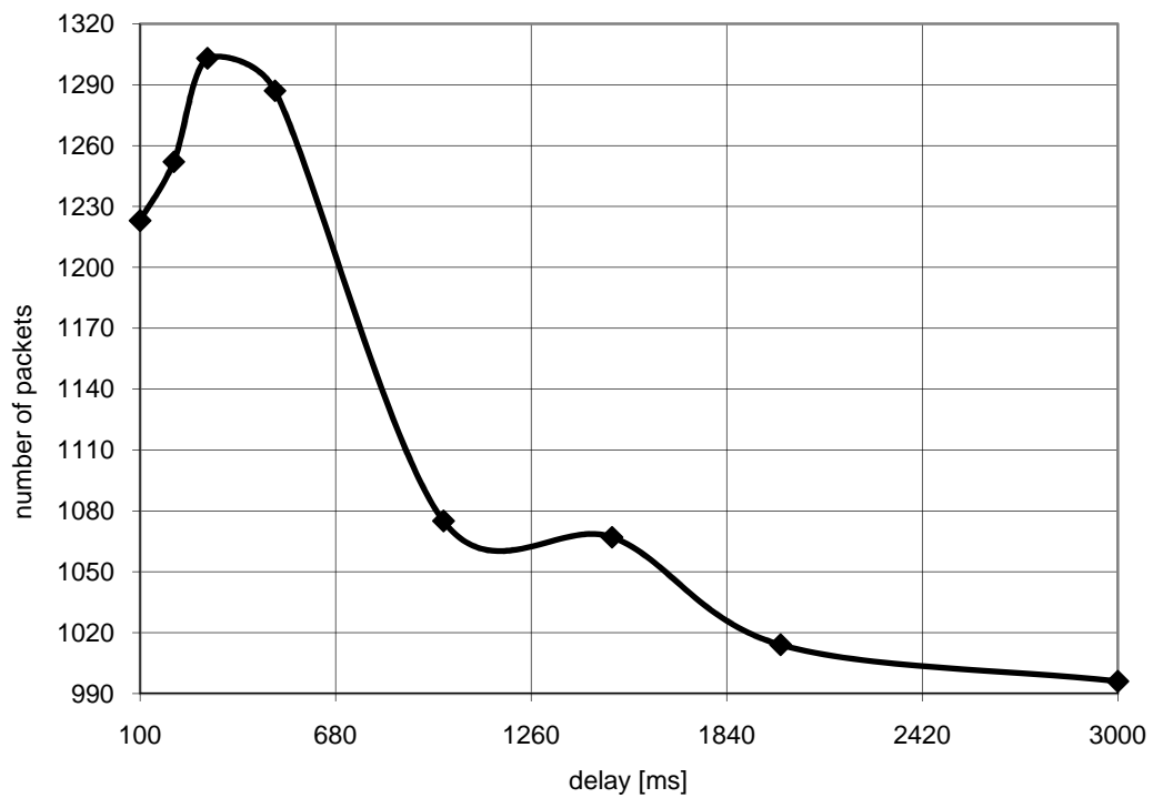
Diagramm aoe_delay2: Age of Empires delay 2
