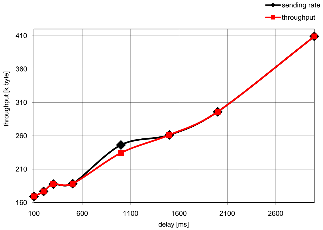
Diagramm q4_delay3: Quake 4 delay 3
