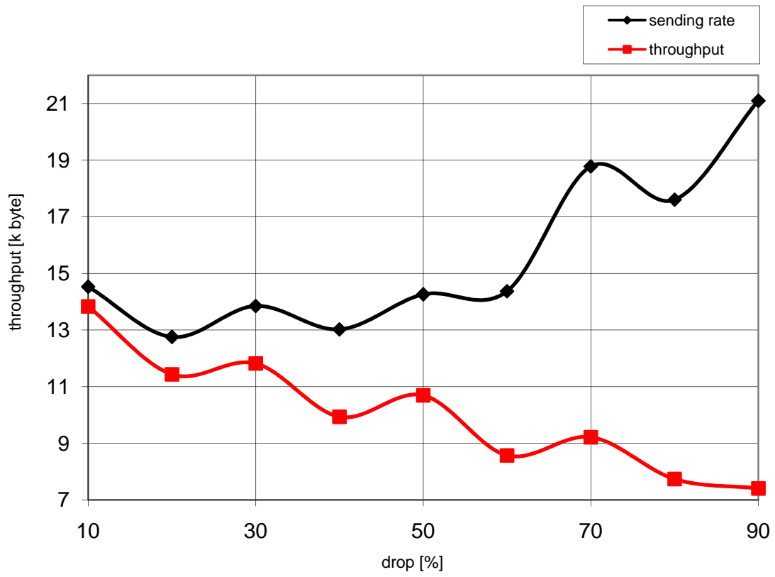
Diagramm aoe_drop3: Age of Empires drop 3
