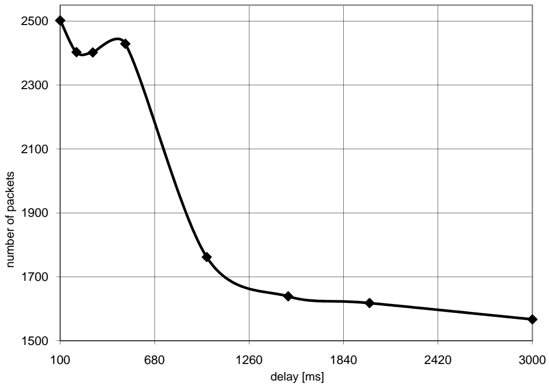
Diagramm fifa_delay2: Fifa 2007 delay 2
