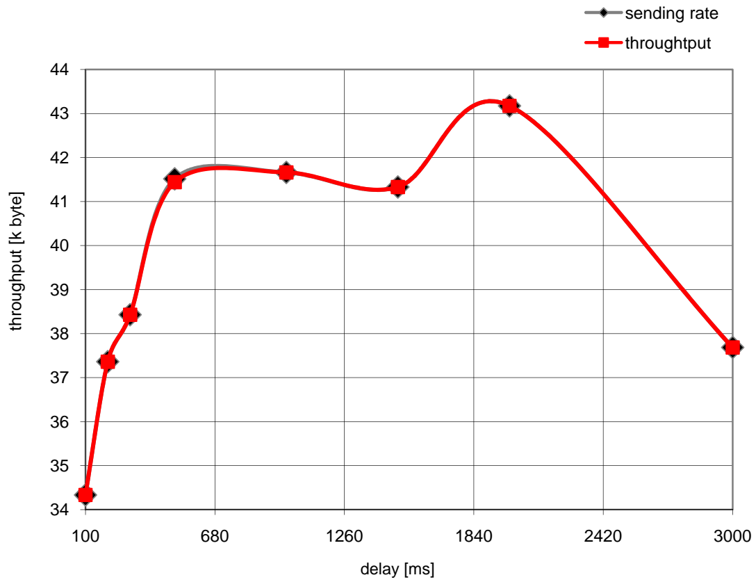
Diagramm dow_delay3: Dawn of War delay 3
