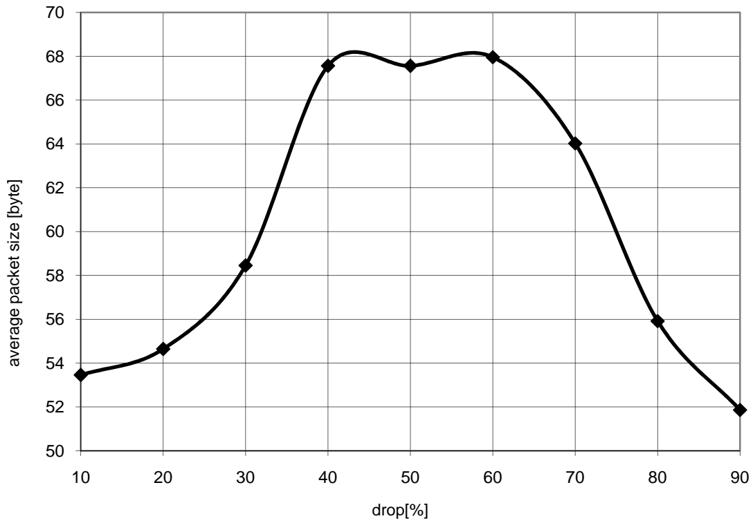
Diagramm dow_drop1: Dawn of War drop 1
