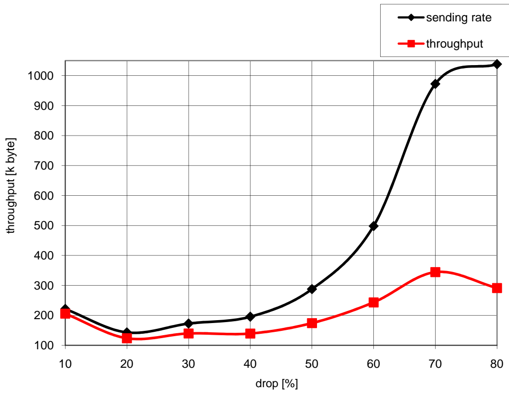
Diagramm fifa_drop3: Fifa 2007 drop 3
