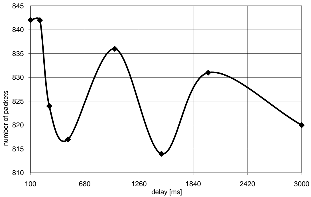
Diagramm dow_delay2: Dawn of War delay 2
