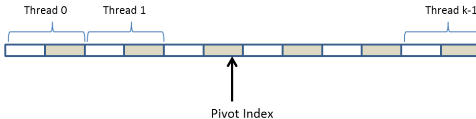
Figure 1. Partition of a[] into k segment, with a number of 'smaller' and 'bigger' than the common Pivot value.
