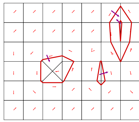
Figure 4: Semi-separatrices
