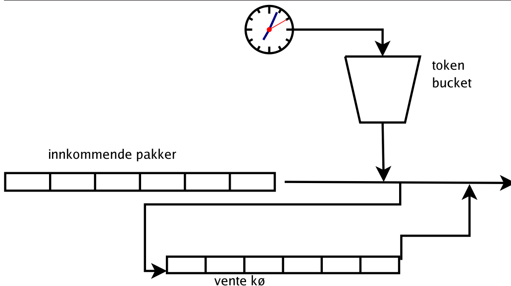
Figur 4.2 token bucket
