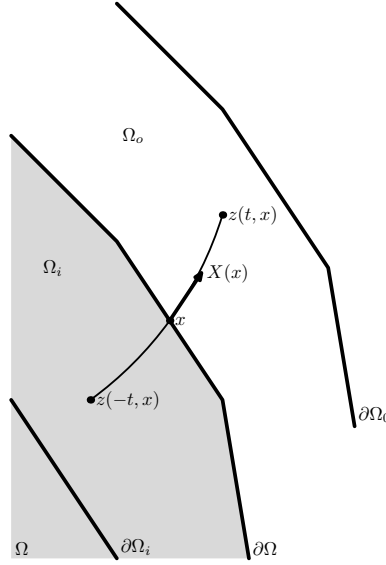
FIGURE 4.1. Extension by reflection
