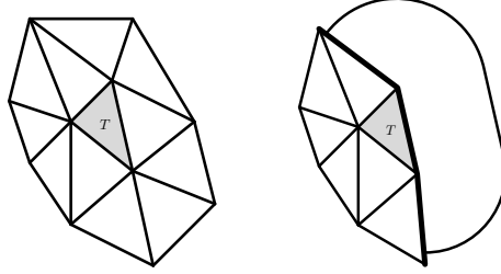
FIGURE 4.2. The macroelement \mathcal{T}_h(T) and the domain T^* associated with the shaded simplex T . To the left T is an interior simplex, while T intersects the boundary, and hence T^* extends outside \Omega , to the right.
