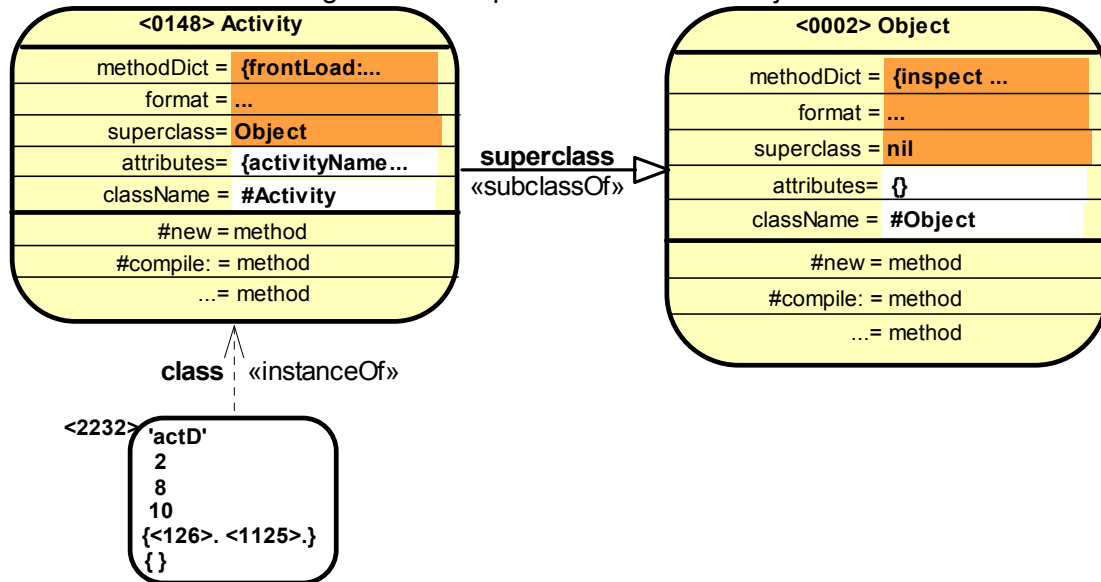
Fig. 13: The implementation of an object.
