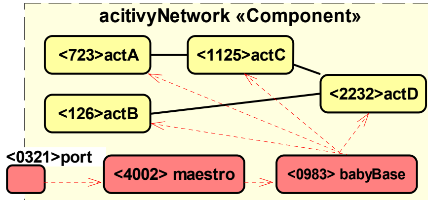
Fig. 14: The objects of the activityNetwork component.
