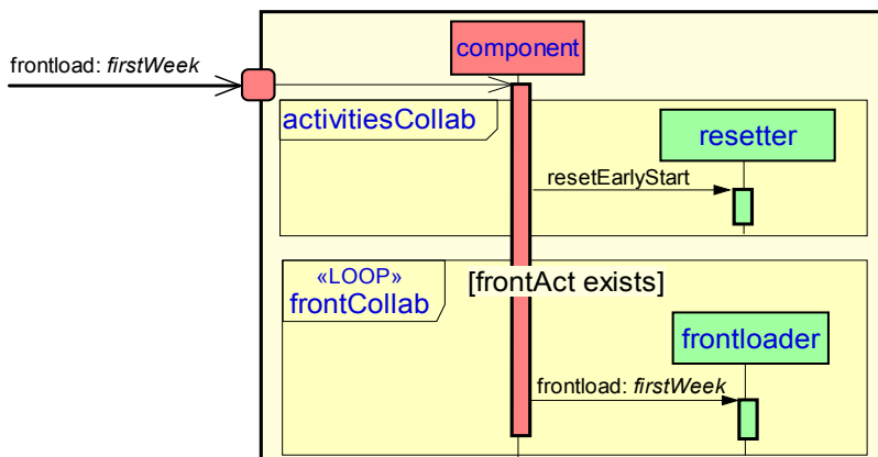
Fig. 8: Frontloading sequence diagram.
