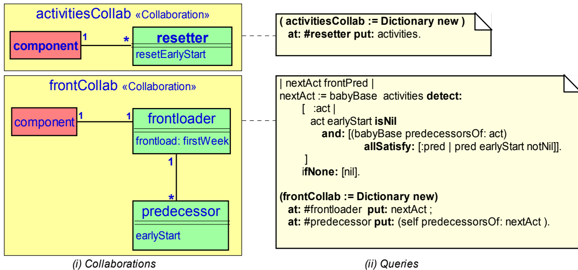
Fig. 9: Frontloading collaborations.
