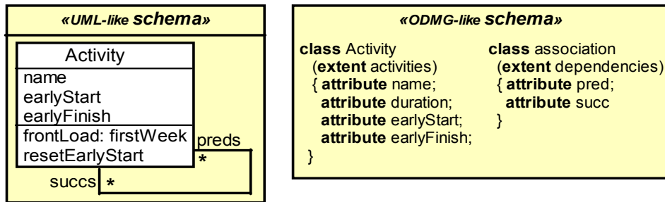
Fig. 5: One simple schema, two languages. .
